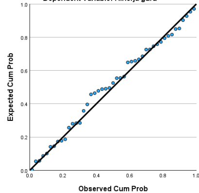
Normal P-P Plot of Regression Standardized Residual Dependent Variable: Kinerja guru
