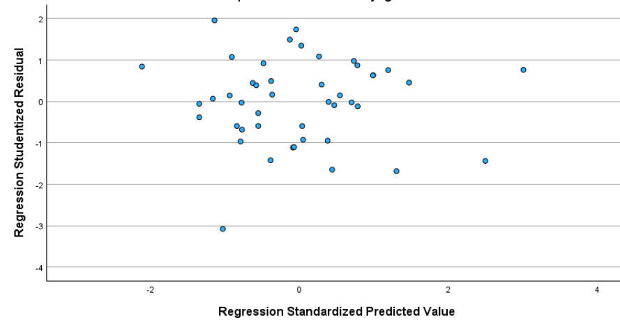
Scatterplot Dependent Variable: Kinerja guru
