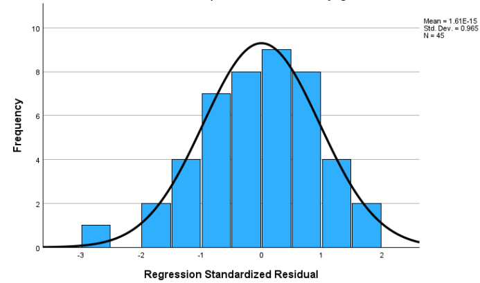
Histogram Dependent Variable: Kinerja guru
